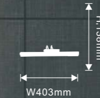
15814 LED 5W 594lm, 6000K 25000h
